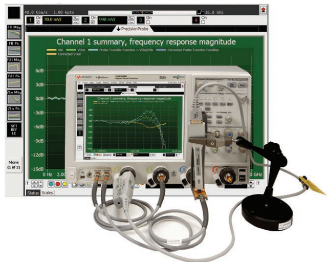
PrecisionProbe uses Keysight's proprietary 200 GHz indium phosphide process to create a fast edge for characterization with PrecisionProbe.
